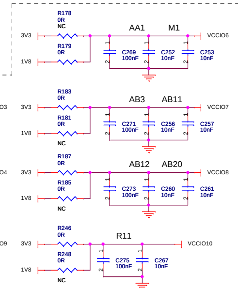
FPGA I/O POWER SUPPLY
